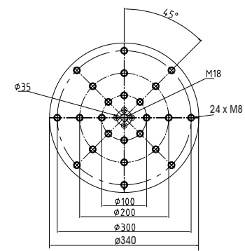
Armature 340 (Standard)
