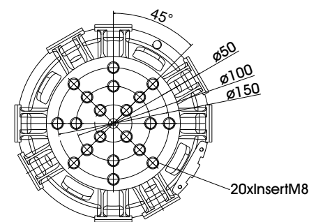
Armature 180 (Standard)
